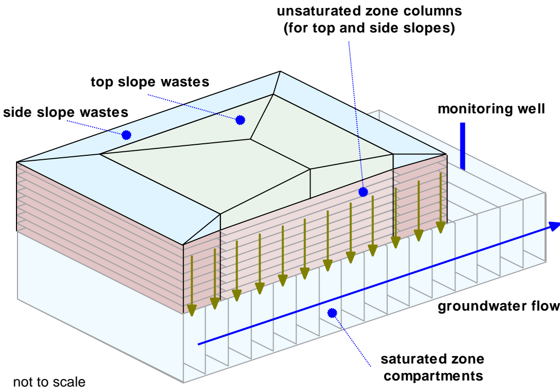
Figure 2: Schematic representation of unsaturated zone and shallow aquifer transport using cell pathways.
