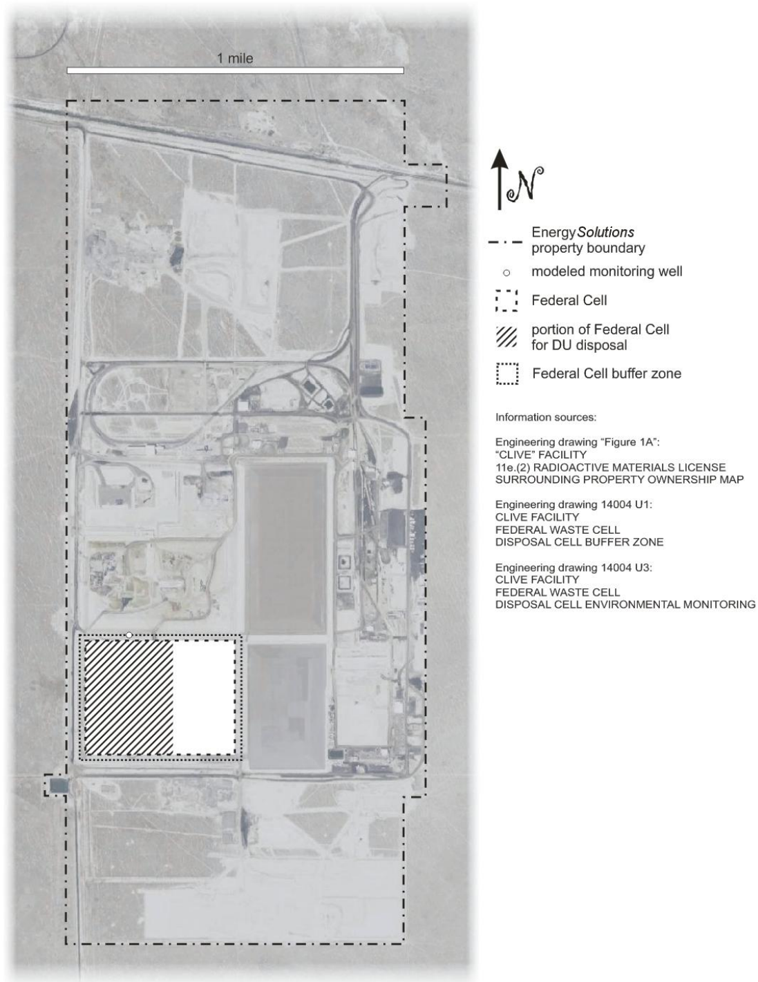
Figure 1. Location and extent of the saturated zone modeling domain including location of the DU waste, the point of compliance monitoring well, the buffer zone of the DU cell, and outer boundaries of property owned and controlled by EnergySolutions.
