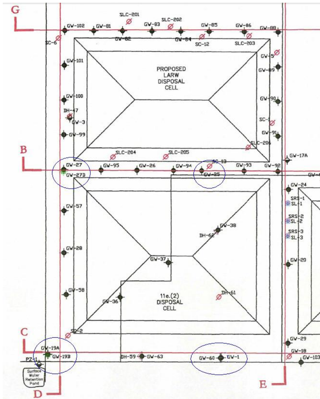
Figure 3. Well locations used for estimating shallow aquifer thickness. Diagram is modified from Envirocare (2004).
